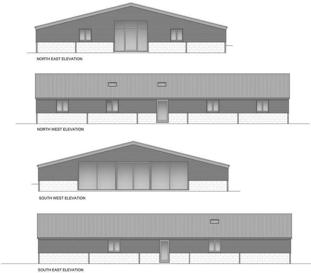
PROPOSED ELEVATIONS
